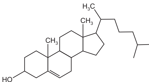
cholesterol
